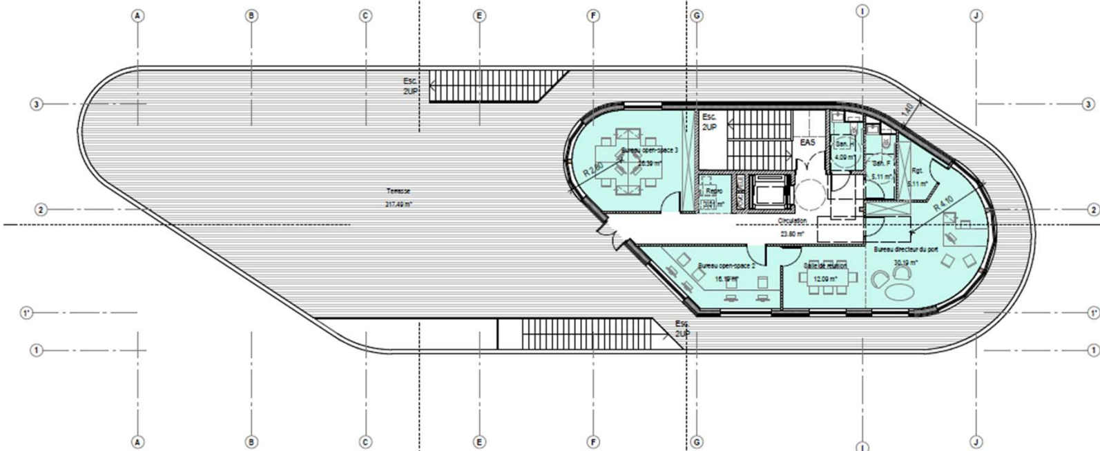
PLAN R+1
